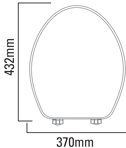
General seat dimensions
