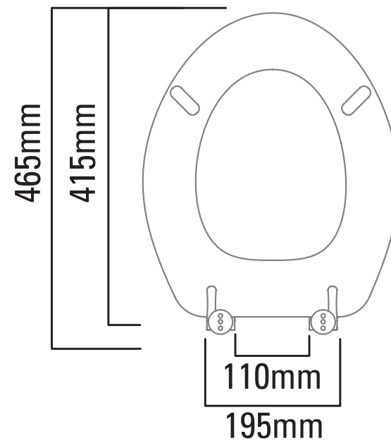
Maximum / Minimum fitting dimensions
