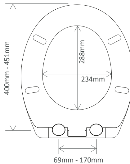
Max/min fixing adjustment
