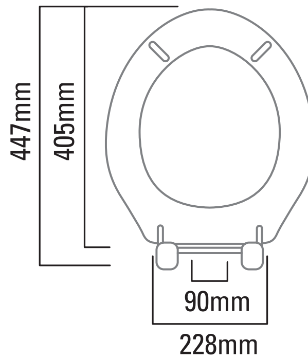
Maximum / Minimum fitting dimensions
